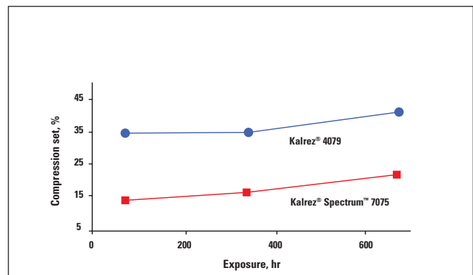
Compression set at 204°C
